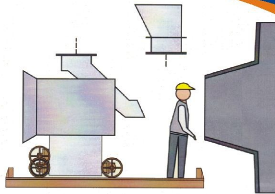
CHUTE IN MOVED ON WHEEL - FOR SAFE ENTRY TO MILL
