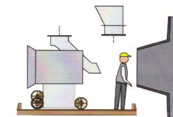
CHUTE IN MOVED ON WHEEL FOR SAFE ENTRY TO MILL
